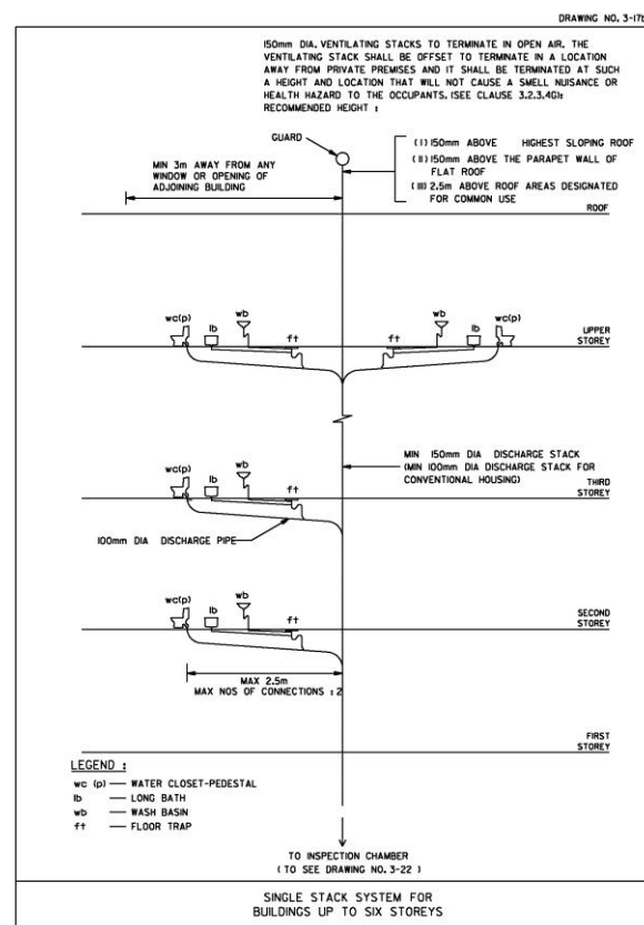
Figure 14 - Single stack arrangement for Buildings up to six storeys. (Separate system above six storeys)
