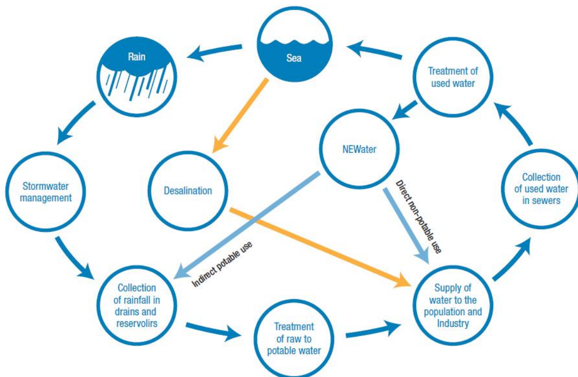
Figure 56 - Singapore's Water Loop (Source; PUB)
