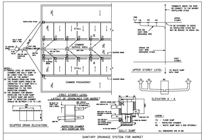
Figure 13 - A Drawing illustrating the drainage system in a Market.
