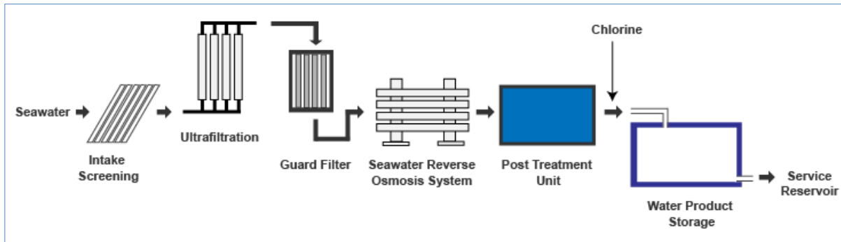
Figure 72 - Schematic flow of Desalination Process (Source: Hyflux)
