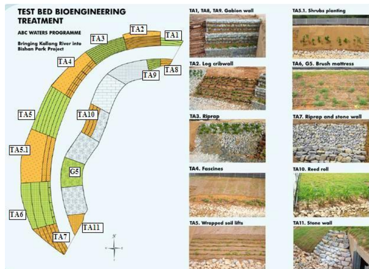
Figure 33 - The Bio-engineered riverbed (up) and Biotope system for treatment using natural materials. (right)
