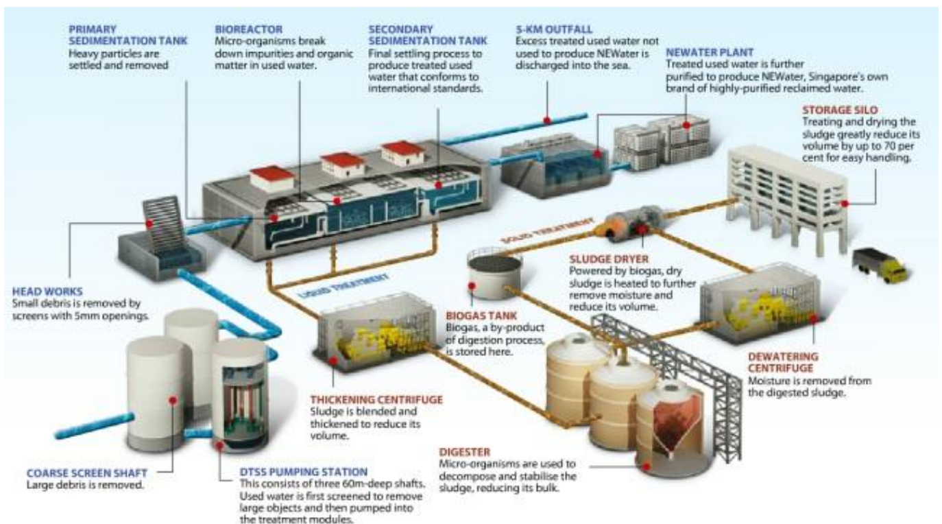
Figure 65 - The Schematic Flow-Chart of DTSS & NEWater
